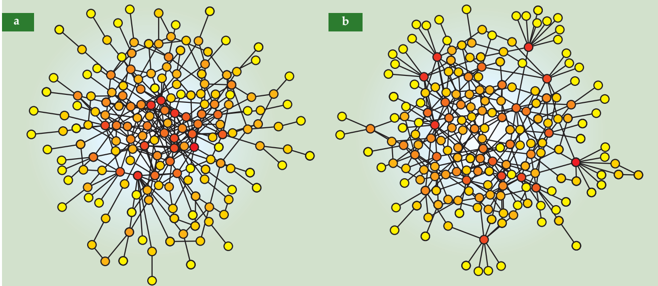
Figure 4. Two networks with the same distribution of node degrees but different degree correlations. Network (a) is positively correlated, whereas (b) is negatively correlated. The nodes are color coded to emphasize their degrees (yellow for low degree, red for high degree). The high-degree nodes clump together in network a but are more spread out in network b. A number of the hub-and-spoke formations characteristic of negatively correlated degrees—created when a high-degree node connects to a lot of low-degree ones—are visible around the edges of network b.
